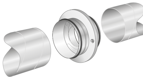
Figur 1. Montering.
