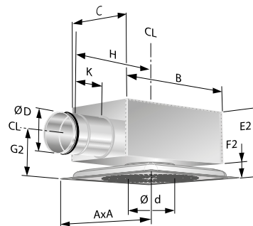
Figure 7. LOCKZONE Ceiling with ALS. Low building height.
