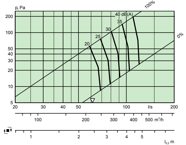
LOCKZONE C 250-500+ALS 200-250 – One step
