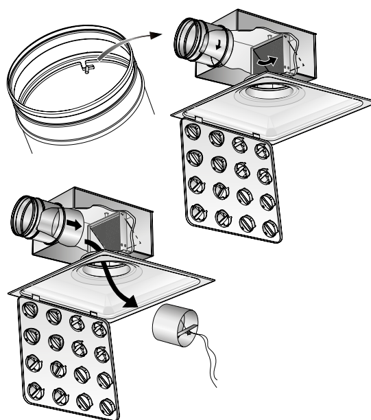
Figure 4. Damper removal.
