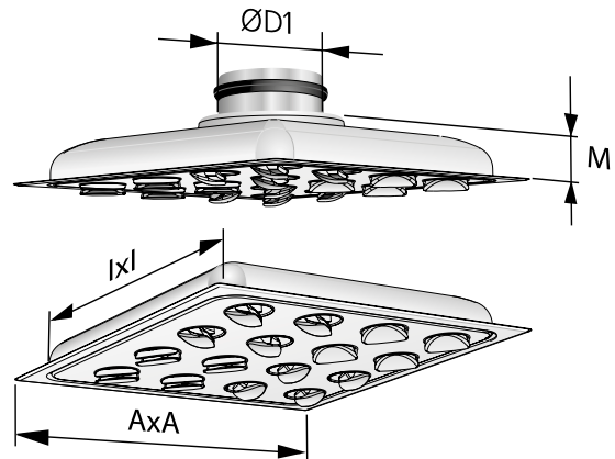
Figure 5. EAGLE Ceiling
