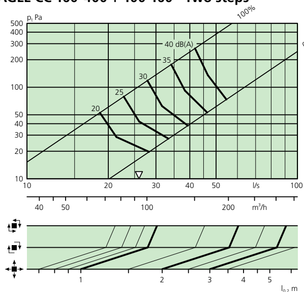
EAGLE CC 160-400 + 100-160 - Two steps
