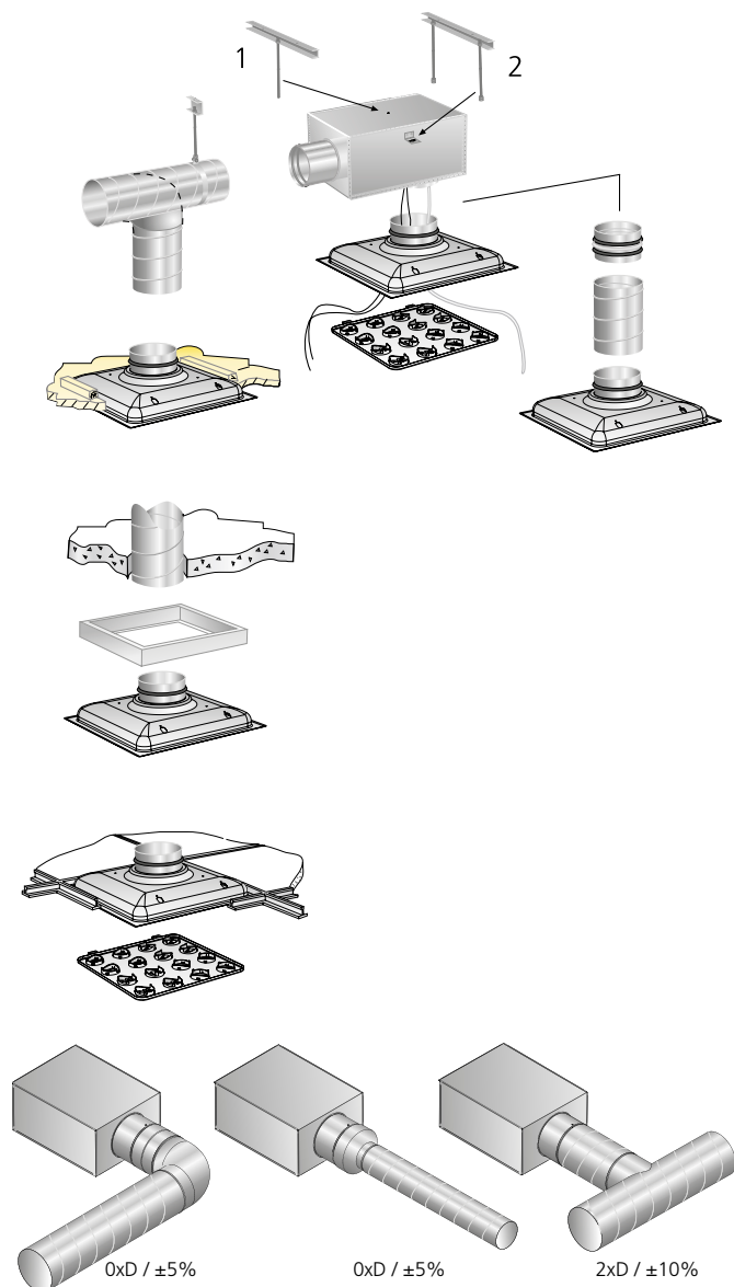
Figure 2. Installation alternatives.
