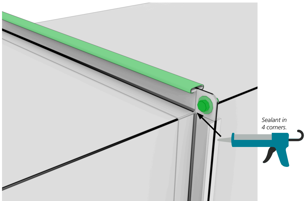
Figure 4. Installation of Euroflange.
