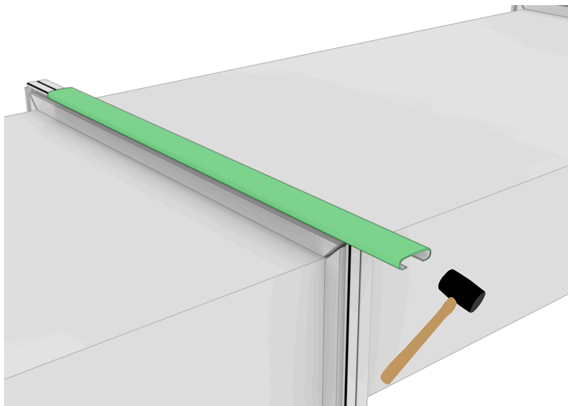
Figure 2. Installing the guide rail.
