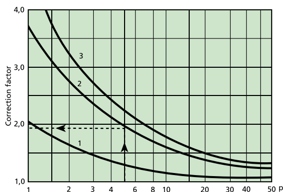
Diagram 1. Correction for different connection
