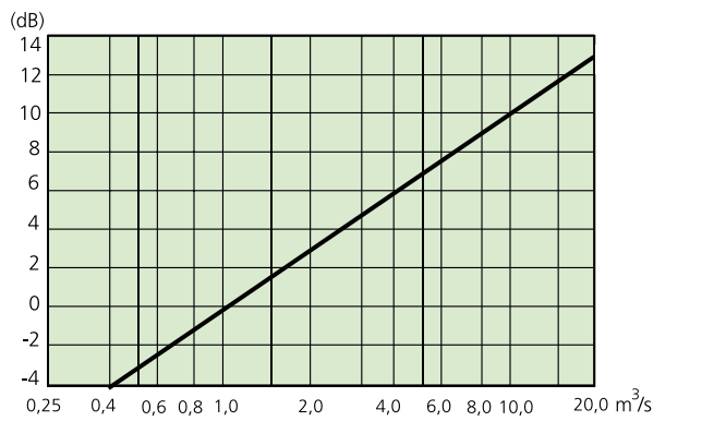
Diagram 2. Correction for airflows other than 1 m³/s
