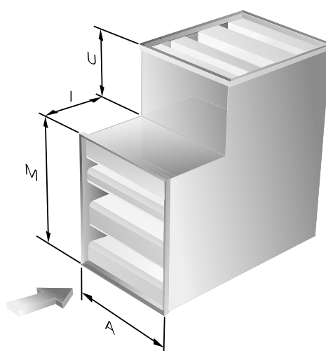
Figure 4b. Vertical installation: M dim. corresponds to the height of the duct. A dim. corresponds to the width of the duct.
