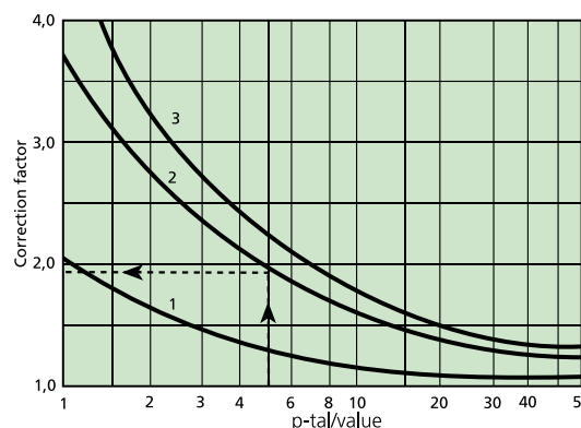
Diagram 1. Correction for other airflows
