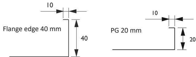
Duct connection
