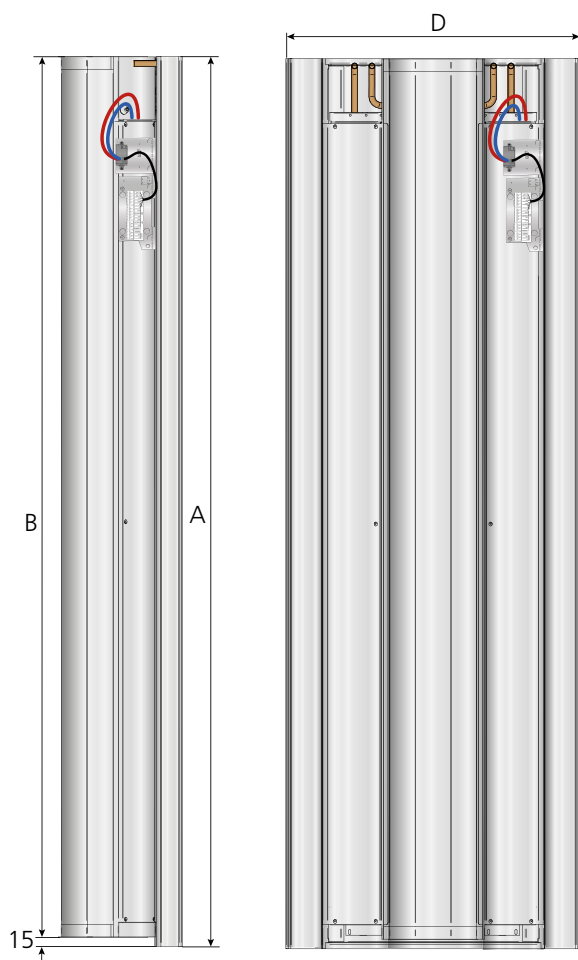
Figure 13. Dimension sketch - full size
