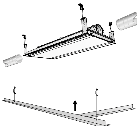
Figure 18. Suspension variant with mounting brackets and threaded rods respectively.
