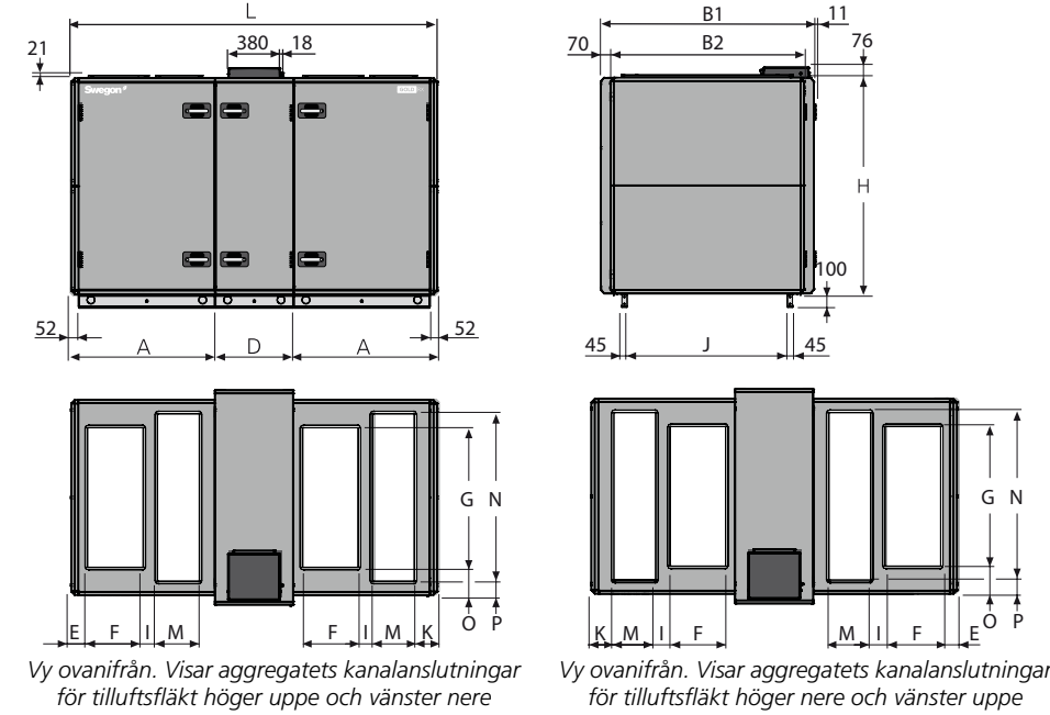
GOLD RX Top 014+/020+
