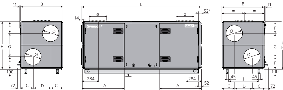
SILVER 04/05, common casing
