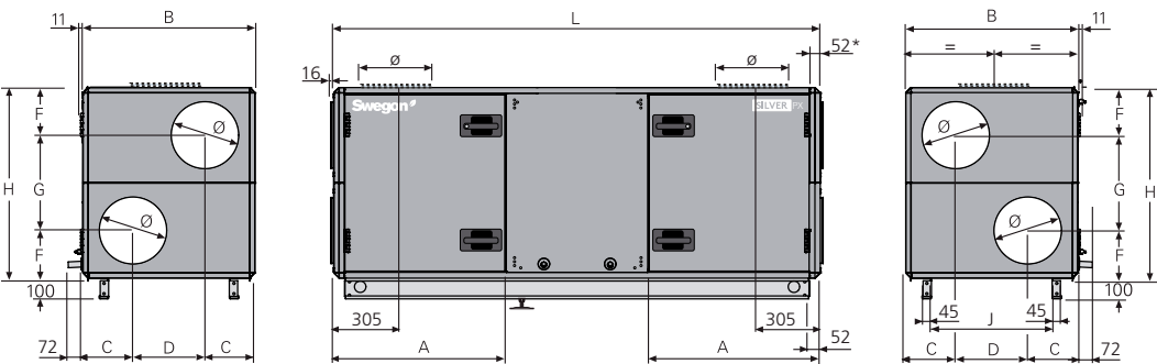
SILVER 07/08, common casing
