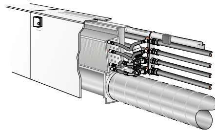
Figur 2. Installation.
