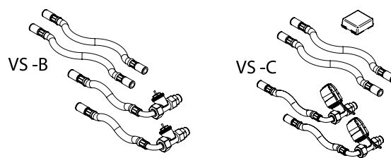
Figur 7. Ventilset VS.
