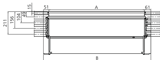
Figure 11. View: front.
