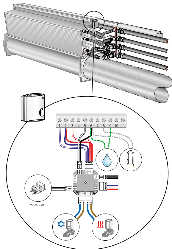
Figure 18. Control equipment LUNA. For particulars on how to wire the electric heating, see the separate installation instructions at www.swegon.com
