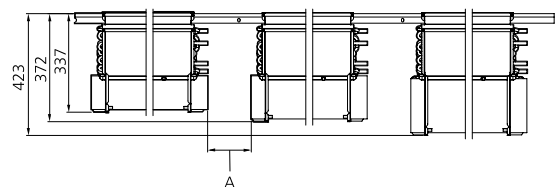
Figure 13. Assembly area.
