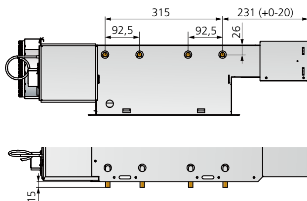
Figure 23. Dimensions suspension
