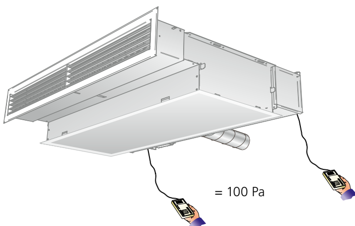
Figure 19. Location of measuring hoses
