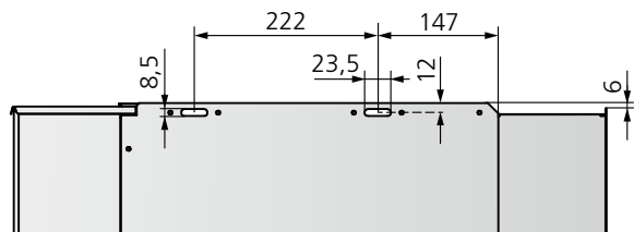
Figure 20. Dimensions suspension
