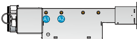
Figure 22. Water connection on the right-hand side (R). A1 = Cooling water, supply B1 = Heating water, supply A2 = Cooling water, return B2 = Heating water, return
