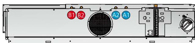
Figure 25. Water connection, Rear edge (WB) A1 = Cooling water, supply B1 = Heating water, supply A2 = Cooling water, return B2 = Heating water, return
