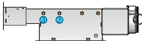
Figure 24. Water connection on the left-hand side (L). A1 = Cooling water, supply B1 = Heating water, supply A2 = Cooling water, return B2 = Heating water, return
