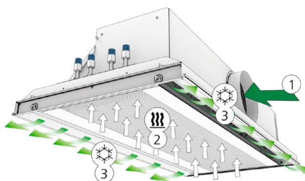
Figure 4. Neutral operation.
