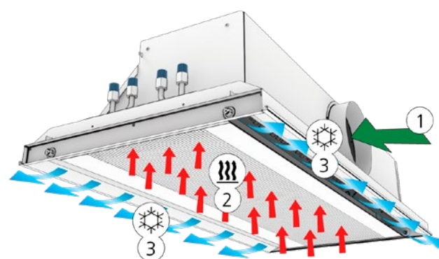
Figure 2. Cooling operation.
