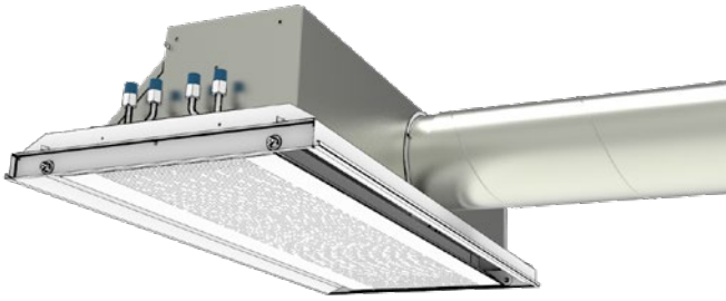
Figure 11. Example with straight, horizontal air connection.
