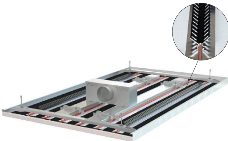
Activated A11-S ceiling panels are suitable for use with Convactor Wings.
