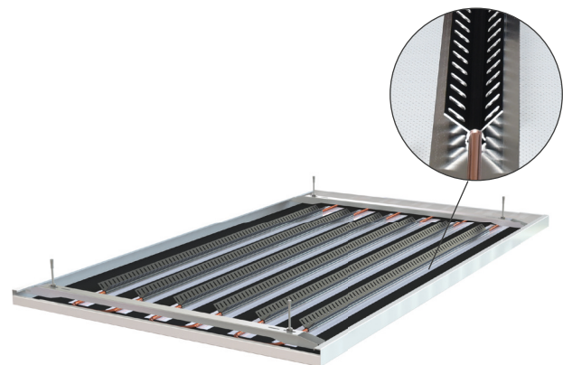
Activated A11-S ceiling panels are suitable for use with Convactor Wings.
