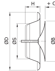
Supply Valve VA
