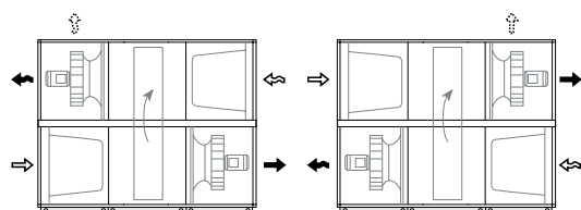
Supply air fan, right, lower level
