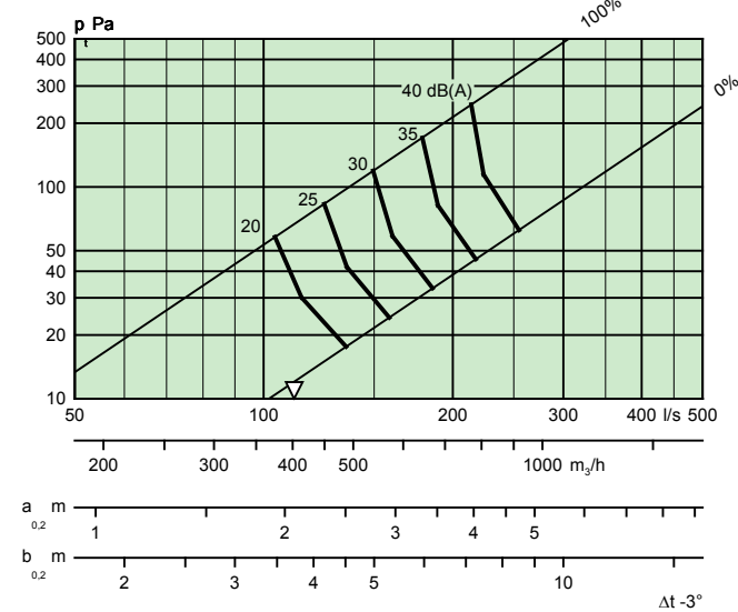
DVC 250 + REG
