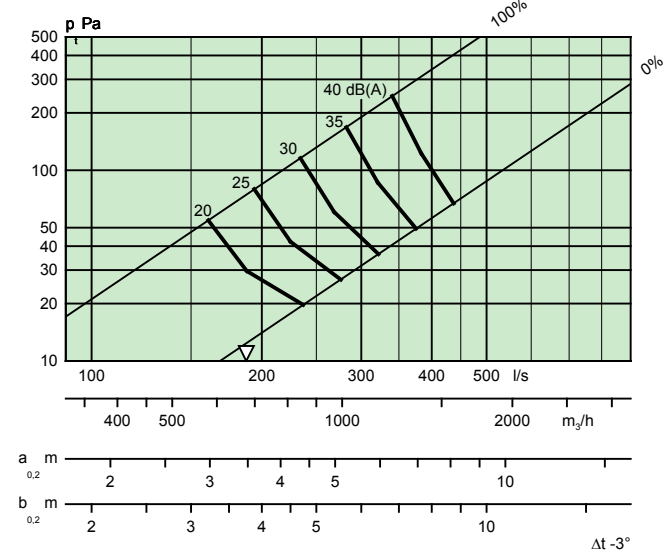
DVC 315 + REG
