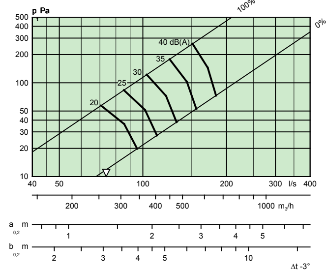
DVC 200 + REG
