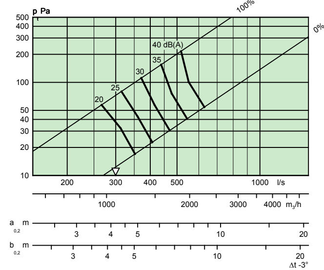
DVC 400 + REG
